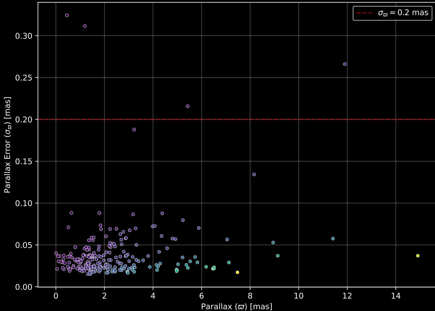
APOGEE DR17 Field: [K2_C10_279+61] Parallax Quality (n= 224)
