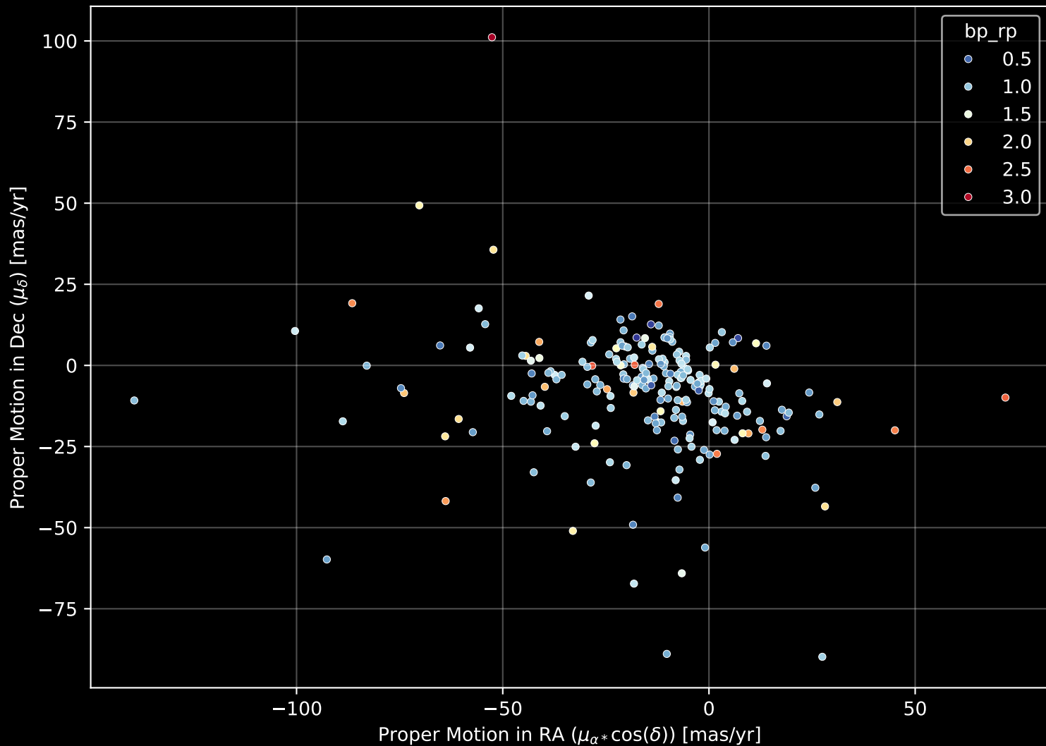
APOGEE DR17 Field: [K2_C10_279+61] Proper Motion Diagram (n= 224)
