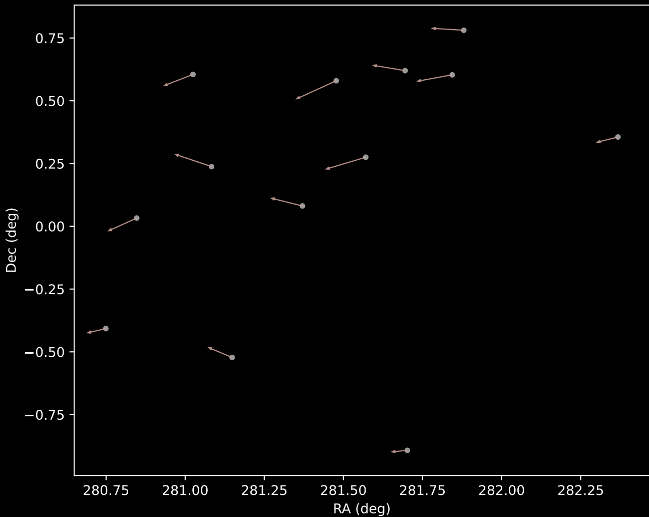
APOGEE DR17 Cluster 11 Proper Motion Vectors (n=13)
