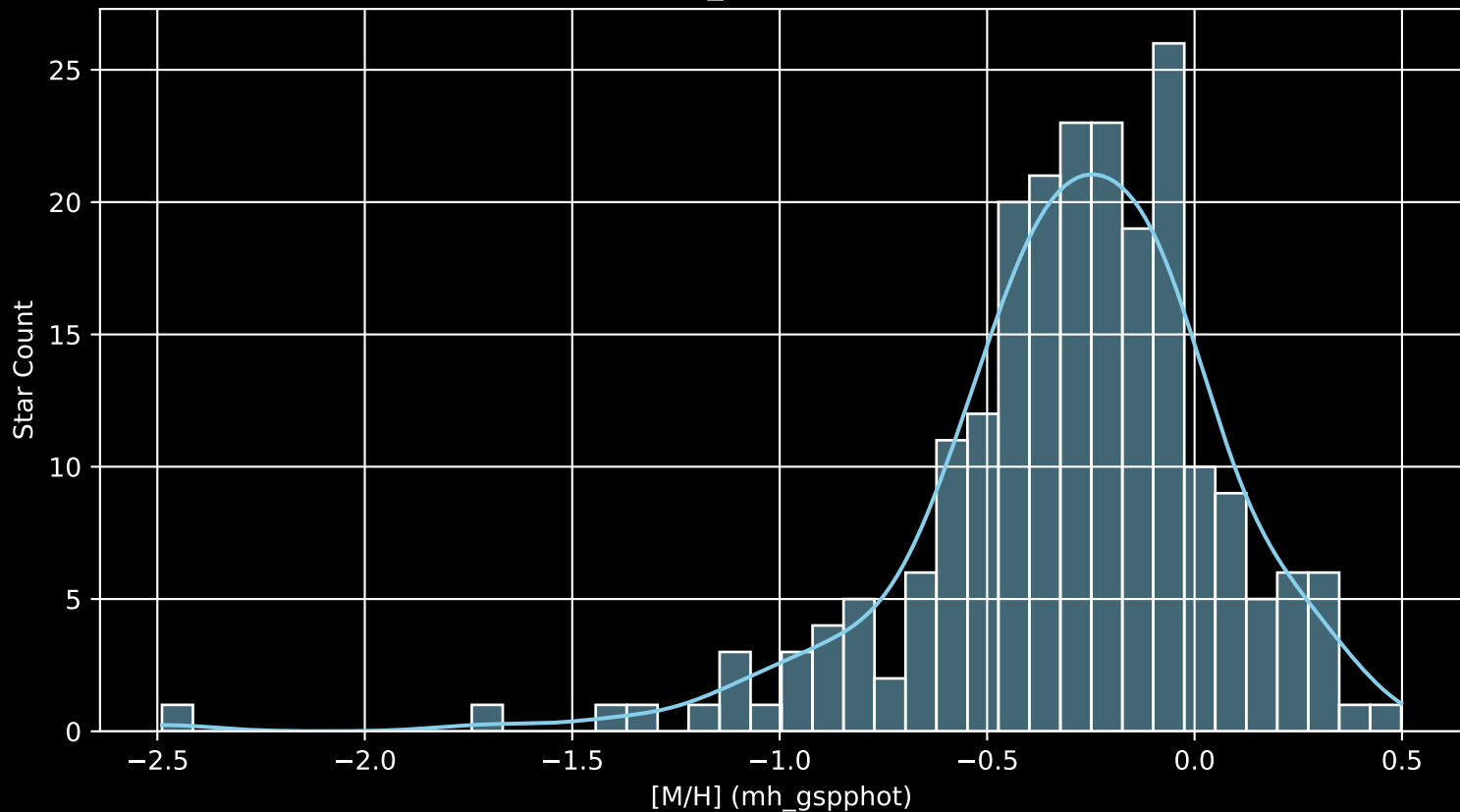
APOGEE DR17 Field: [K2_C10_279+61 [M/H] (mh_gspphot) (n= 222)
