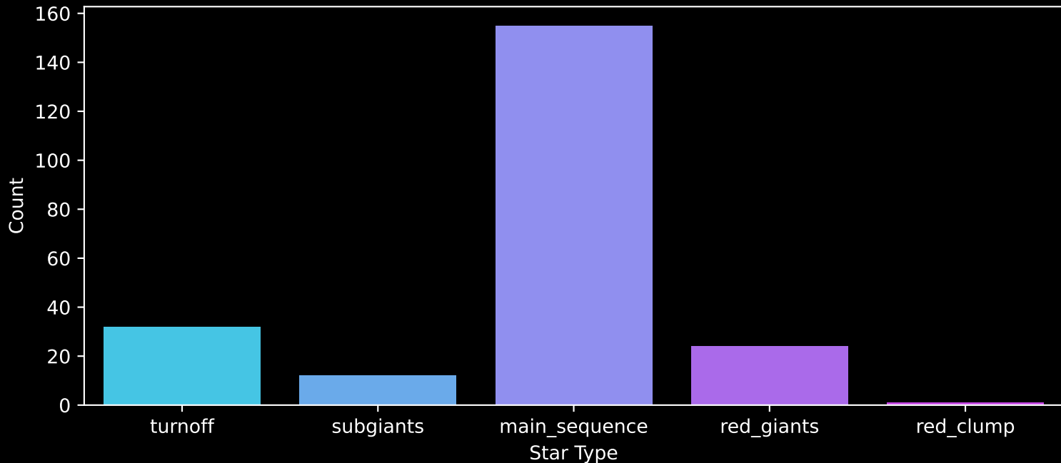
APOGEE DR17 Field: [K2_C10_279+61] Count plot of Star Type
