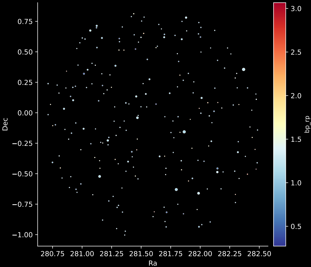
APOGEE DR17 Field: [K2_C10_279+61] Stars: 224
