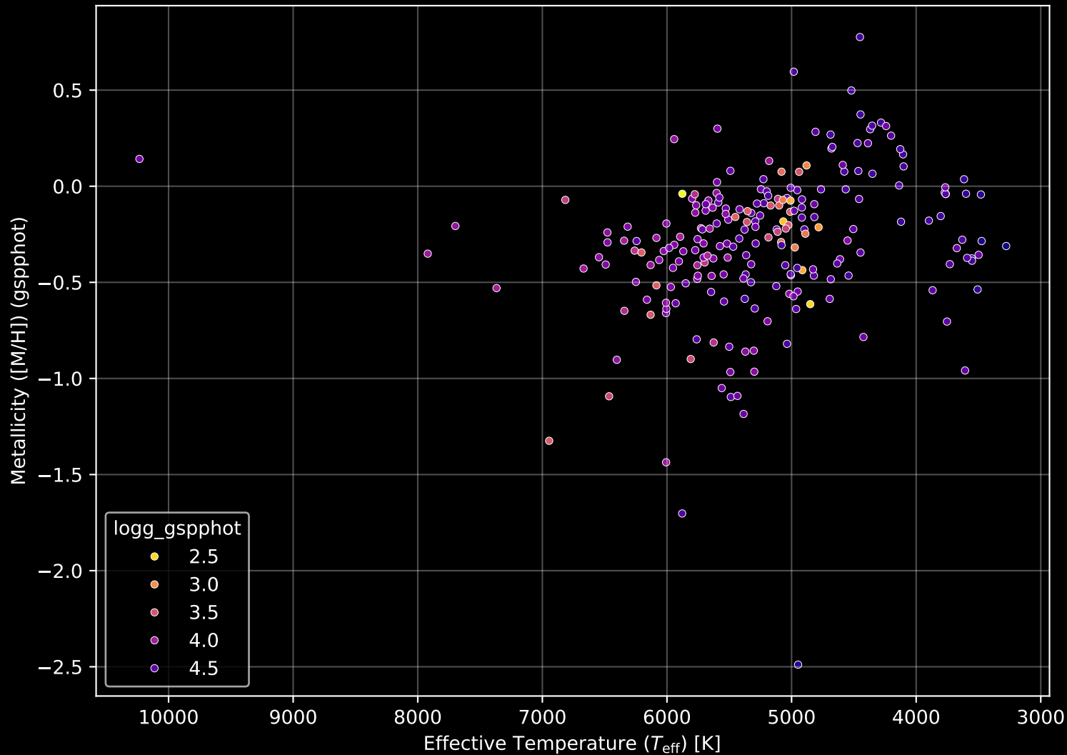
APOGEE DR17 Field: [K2_C10_279+61] Stellar Population Parameters (n= 224)
