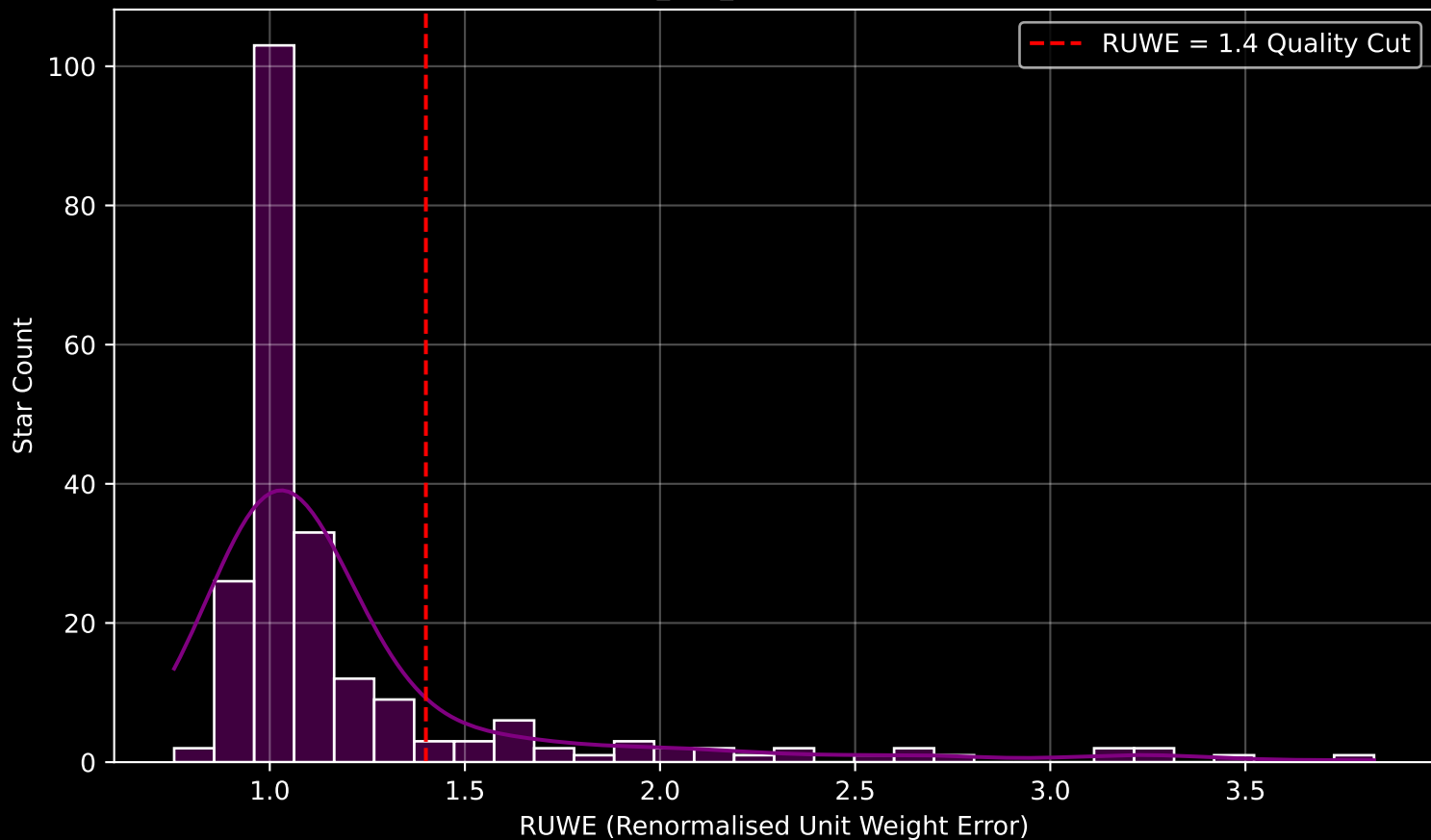
GAPOGEE DR17 Field [K2_C10_279+61] RUWE Distribution (n= 220)
