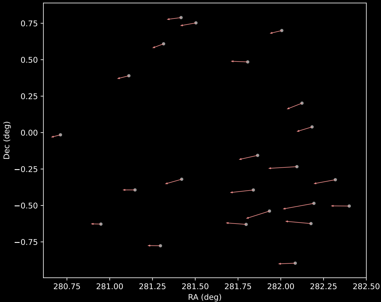
APOGEE DR17 Cluster 7 Proper Motion Vectors (n=23)
